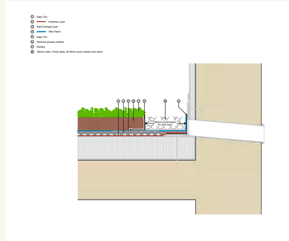
Parapet wall drainage gravel margin
