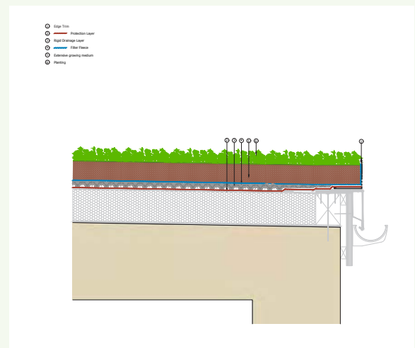
Perimeter drip edge without gravel margin (consider potential wind scour)
