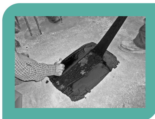
Figure 3 - Cohesive failure (pass)
