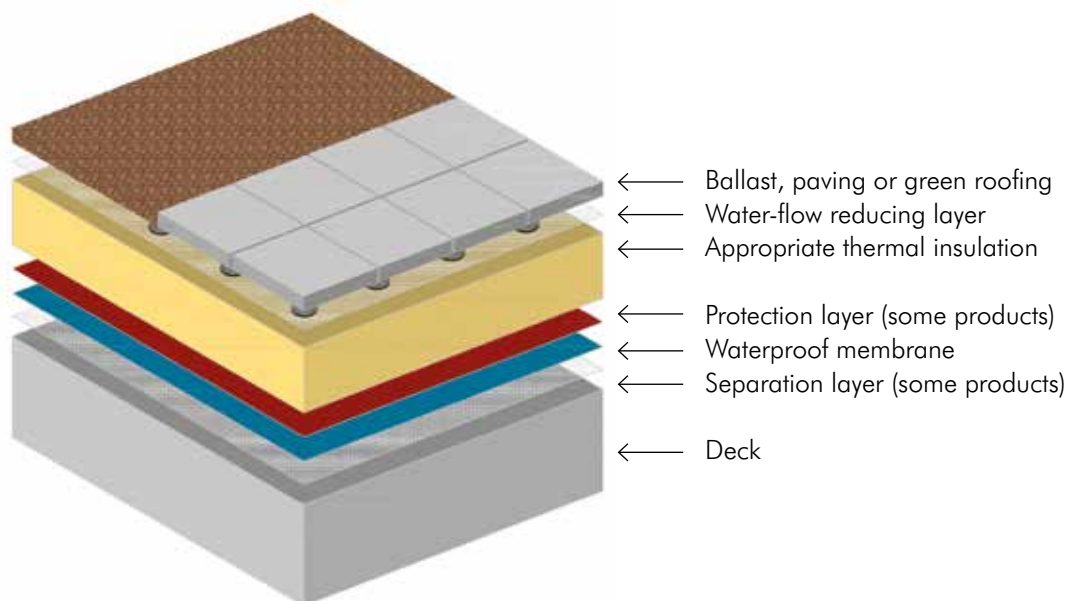
FIG. 2 INVERTED WARM ROOF (SECTION)
