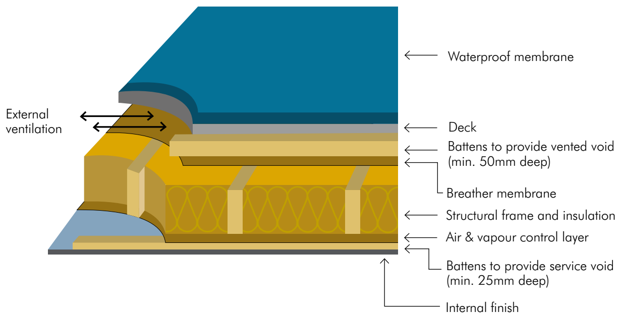
FIG. 4 COLD ROOF (SECTION)
