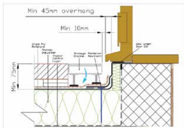
DETAIL 6 LEVEL THRESHOLD – WARM ROOF – PRINCIPLES
