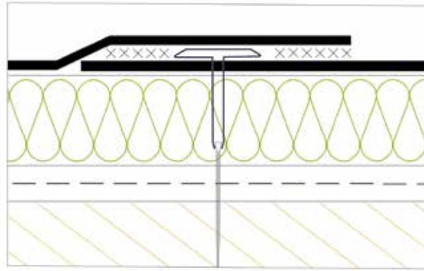
FIG 5B MECHANICAL FASTENING – IN-SEAM FASTENING OF MEMBRANE (ALTERNATIVE FOR EPDM). PLEASE CONSULT MEMBRANE MANUFACTURER FOR SPECIFIC FASTENING REQUIREMENTS.
