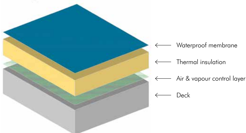
FIG. 1 WARM ROOF (SECTION)
