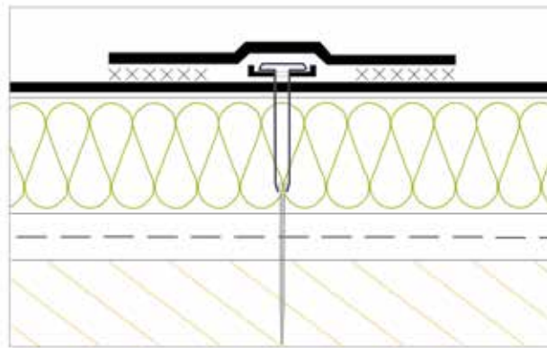
FIG. 6 MECHANICAL FASTENING – LINEAR BAR FASTENING OF MEMBRANE
